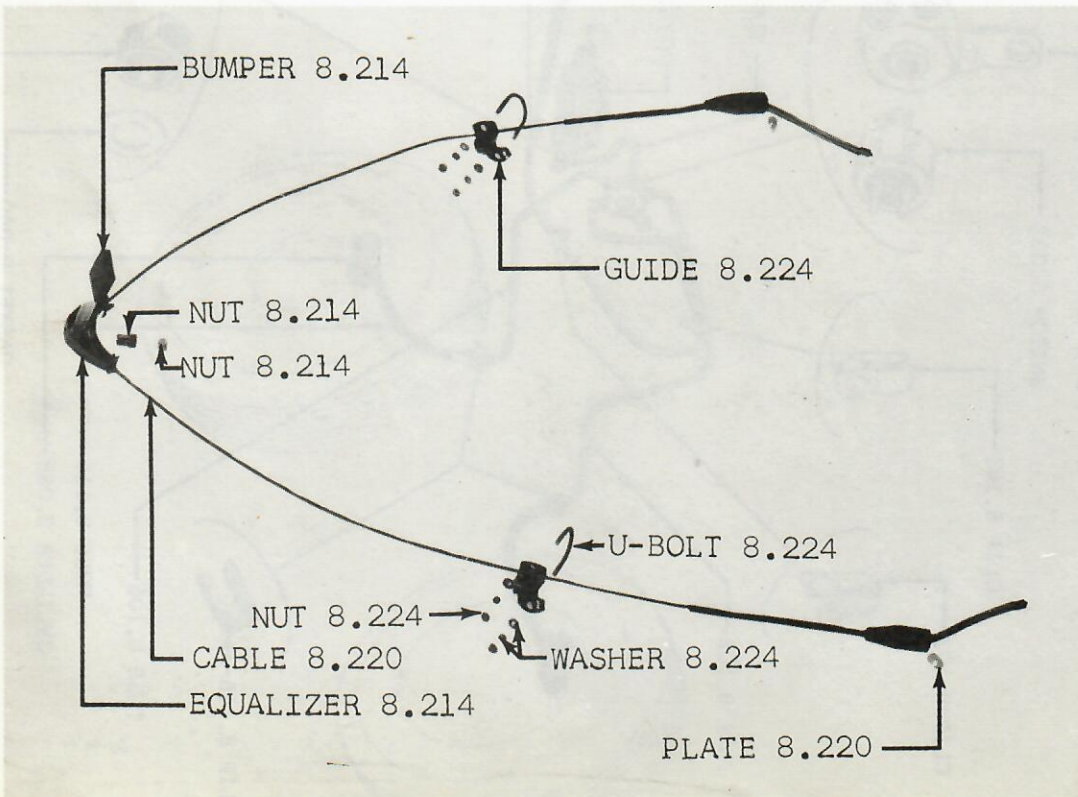
GROUP 8 - FIG. 9 - PARKING BRAKE (YOKE TO DRUM) 10-20-80 (LHD)
