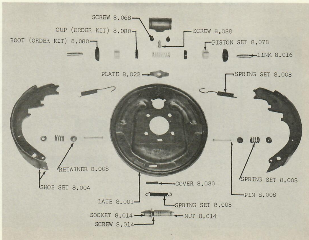
GROUP 8 - FIG. 2D - FRONT BRAKE 20-80 (LAB)
