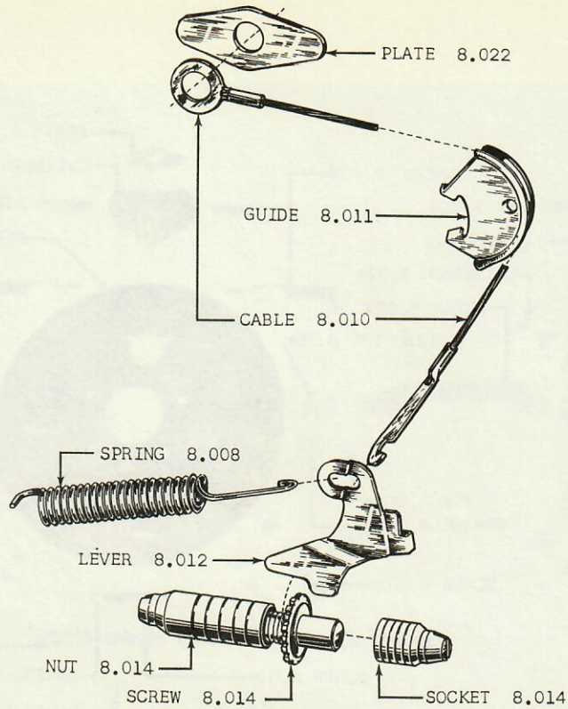
GROUP 8 - FIG. 2C - BRAKE SHOE SELF ADJUSTMENT ASSEMBLY 20-80 (WAB)
