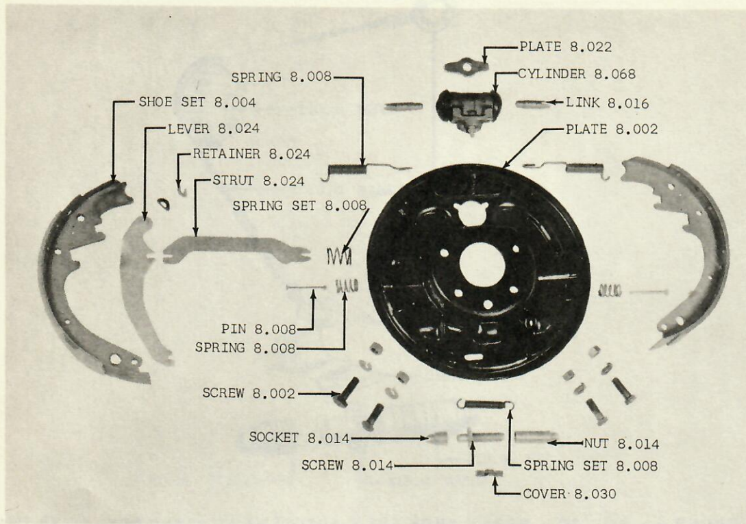
GROUP 8 - FIG. 3 - REAR BRAKE 20-80 (LAB)
