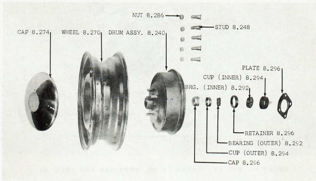
GROUP 8 - FIG. 10 - FRONT WHEEL 01-10-20-80
