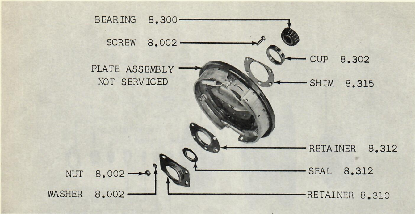
GROUP 8 - FIG. 12 - BRAKE SHIMS, RETAINER AND SEAL 20
