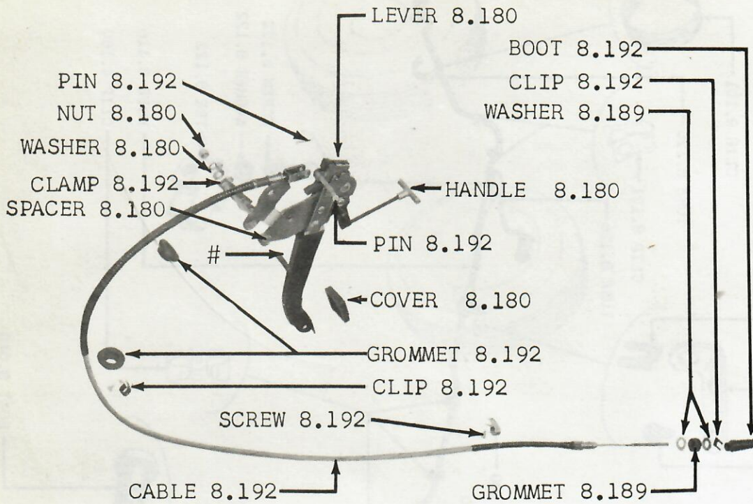
GROUP 8 - FIG. 8 - PARKING BRAKE (PEDAL TO YOKE) 10-20-80 (LHD)
