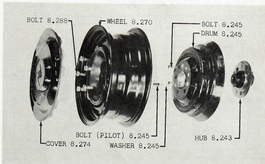
GROUP 8 - FIG. 11 - REAR HUB AND DRUM 20-80
