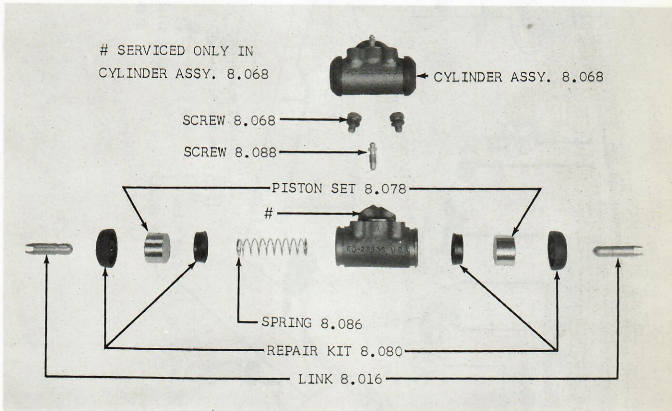
GROUP 8 - FIG. 5 - BRAKE WHEEL CYLINDER 01-10-20-80
