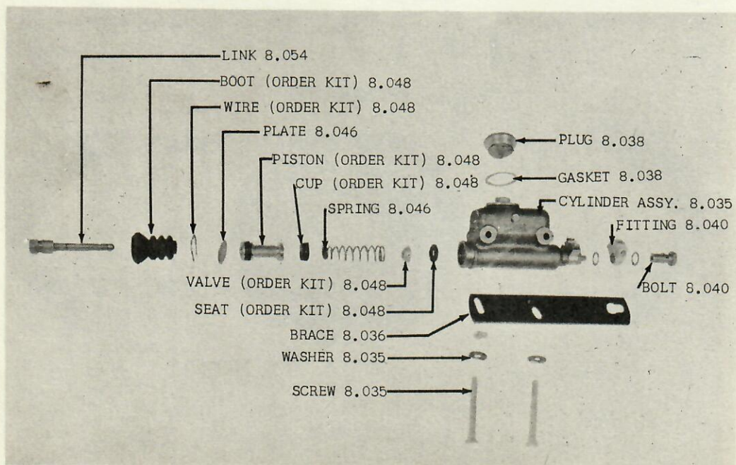
GROUP 8 - FIG. 4 - BRAKE MASTER CYLINDER 01-10-20-80 (LPB)
