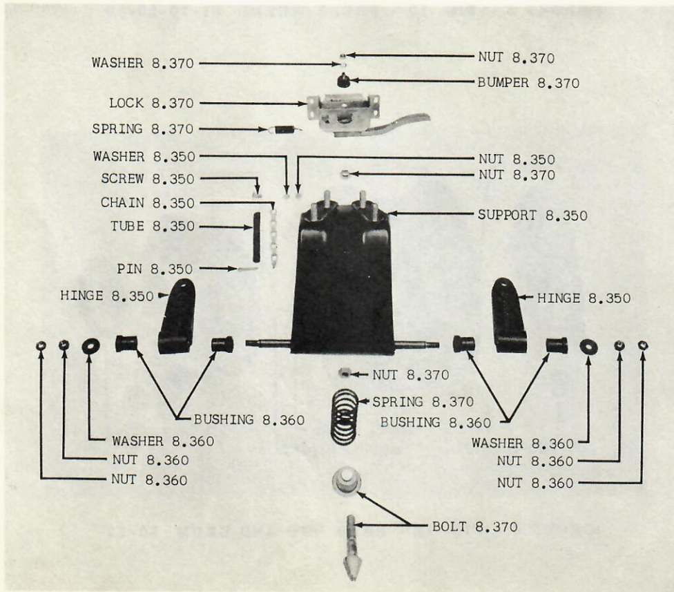
GROUP 8 - FIG. 13 - SPARE WHEEL CARRIER SUPPORT 10-20-80 (WWC)
